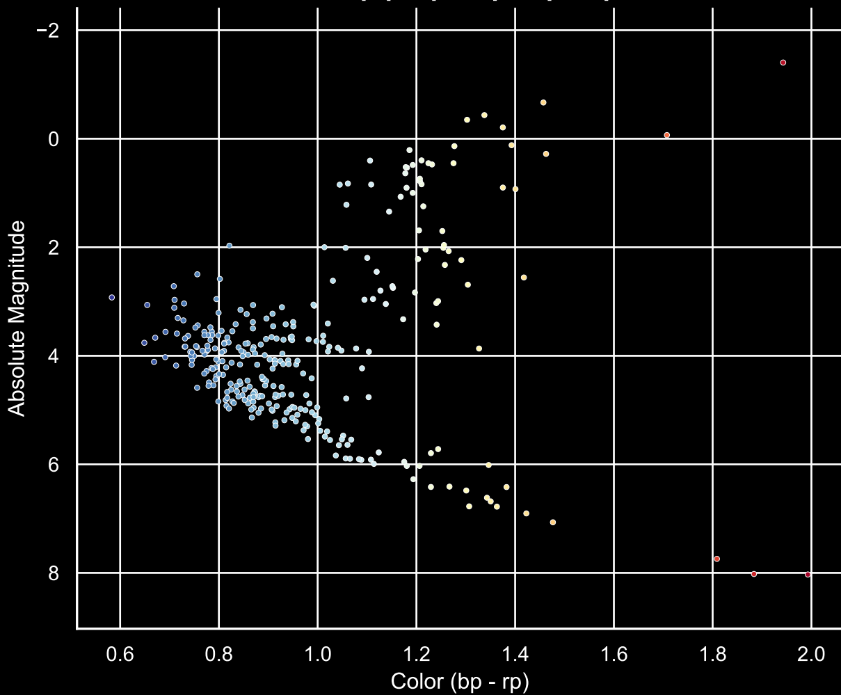
GALAH Hertzprung-Russel Diagram Field [19] Ra [327.89] Dec [-15.64]
