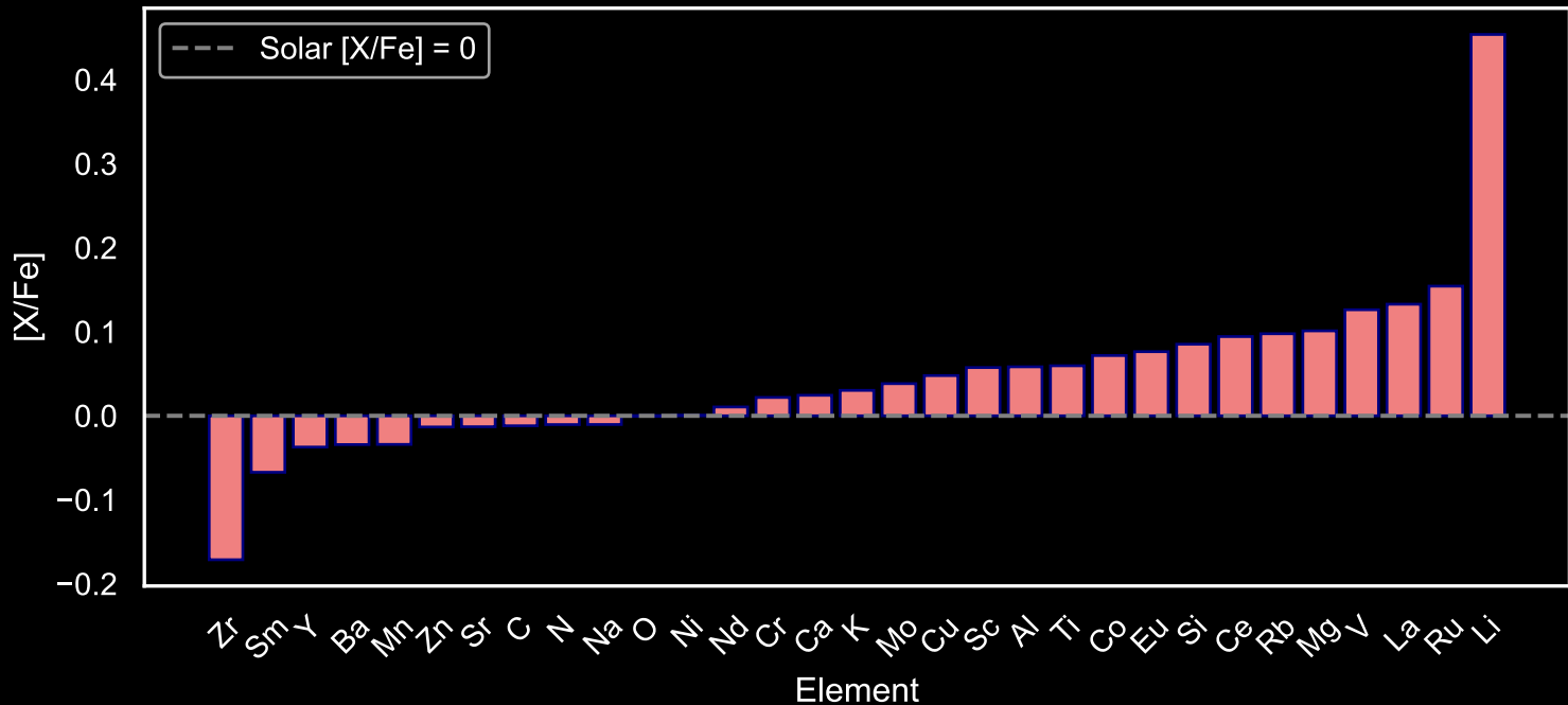
Abundance Pattern for GALAH Main Sequence Stars: Star Field [19] (N=142)
