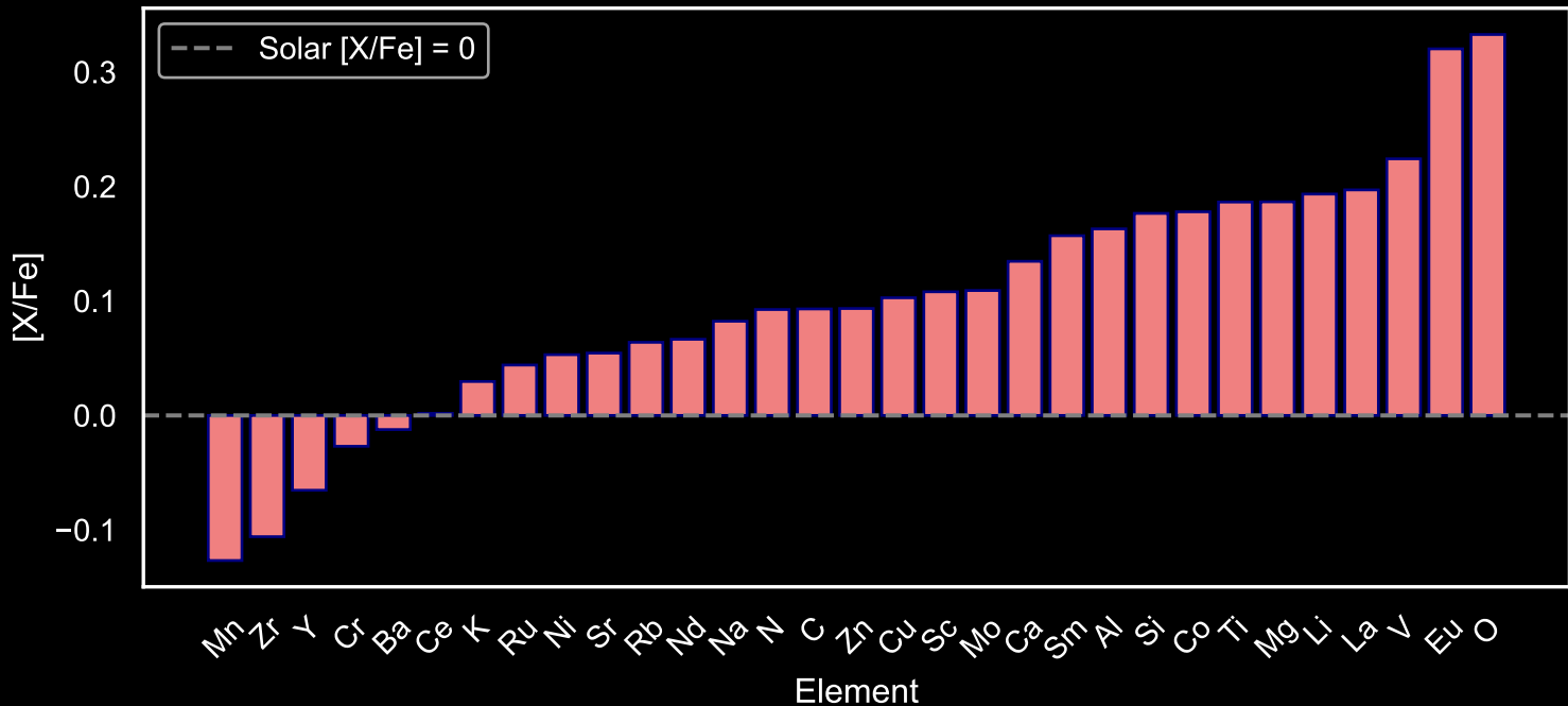
Abundance Pattern for GALAH Red Giants: Star Field [19] (N=61)
