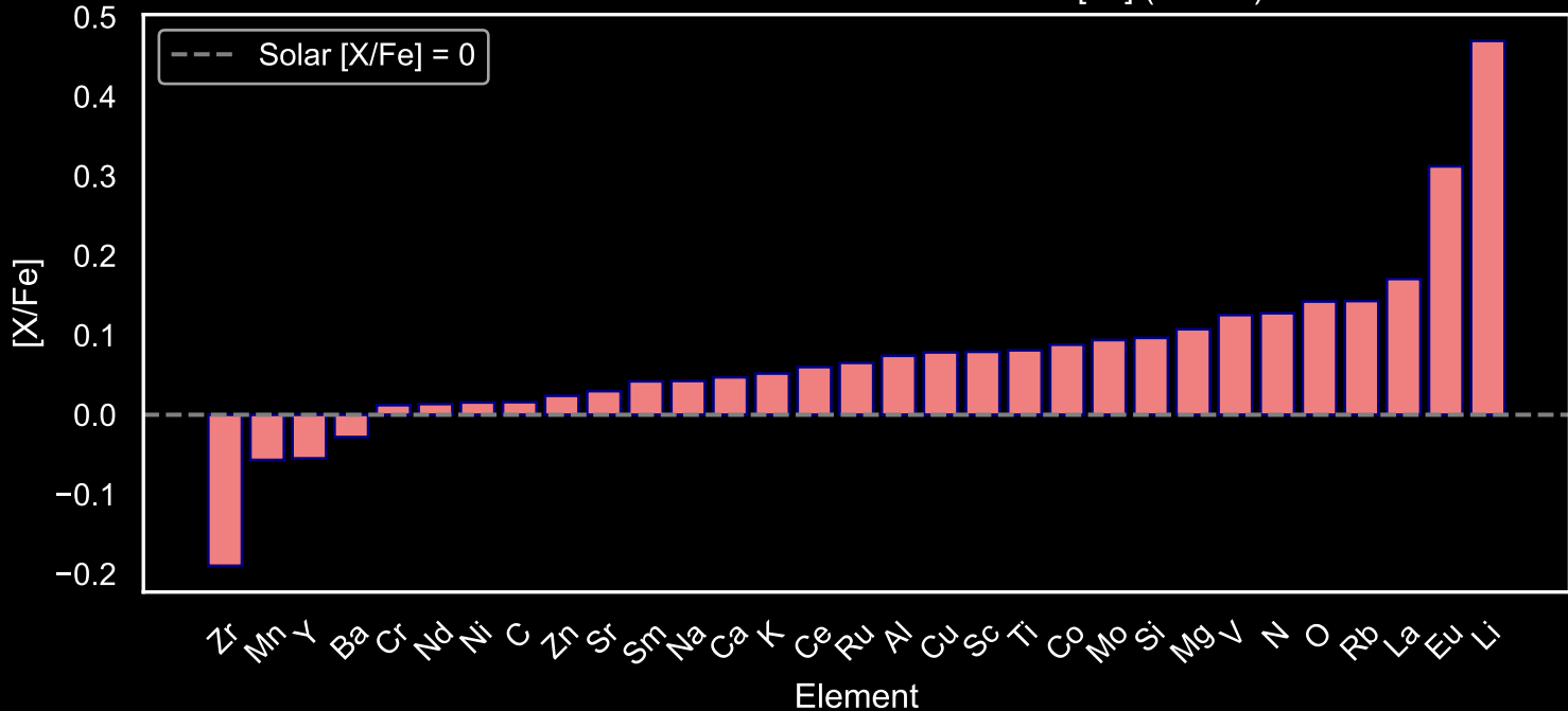
Abundance Pattern for GALAH Star Field [19] (N=311)
