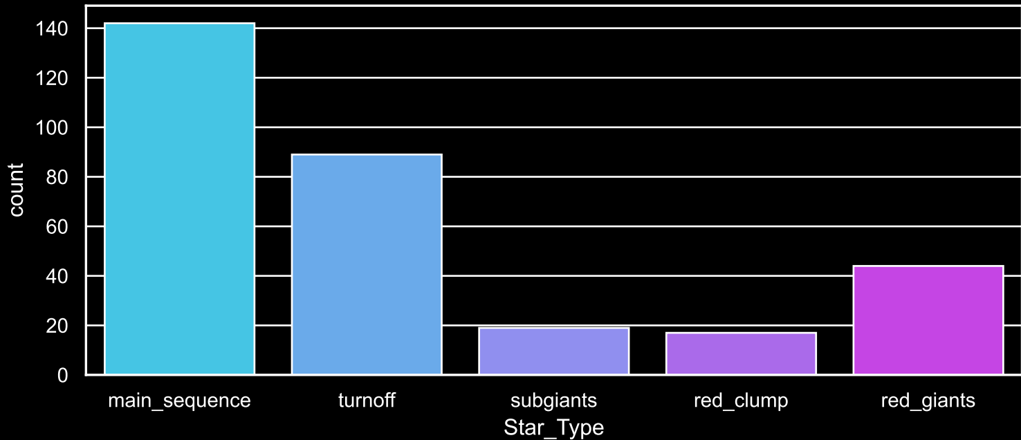
Field [19] Count plot of Star Type
